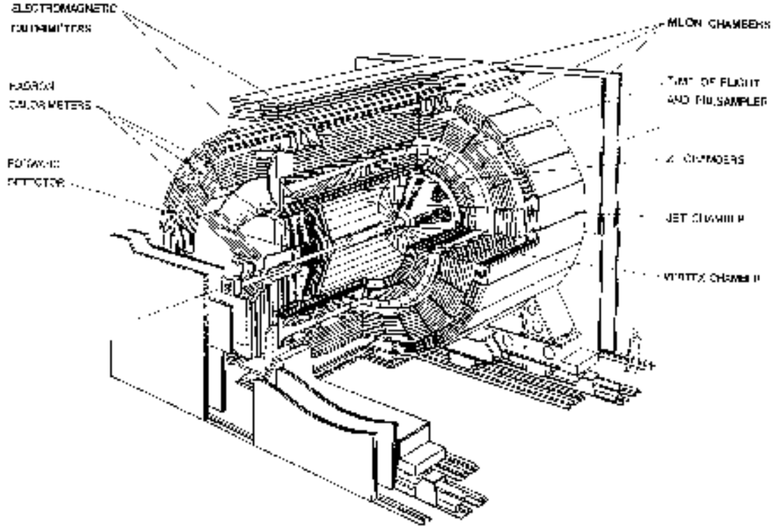
Fig. 2.13: OPAL detector [17].
