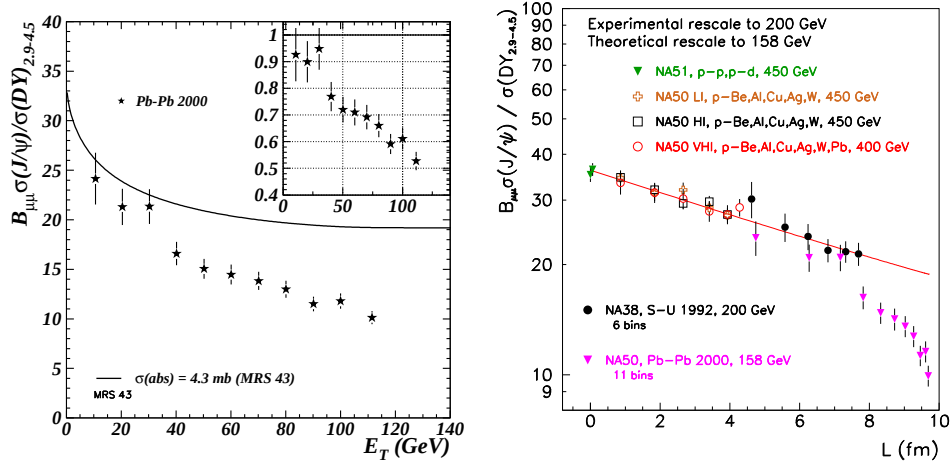
Fig. 7.21: Left-hand side: the (J/\psi)/\text{Drell-Yan} ratio as a function of centrality in Pb+Pb collisions at 158 GeV/nucleon. Right-hand side: the (J/\psi)/\text{Drell-Yan} ratio for several systems, from pp to Pb+Pb, as a function of L .
