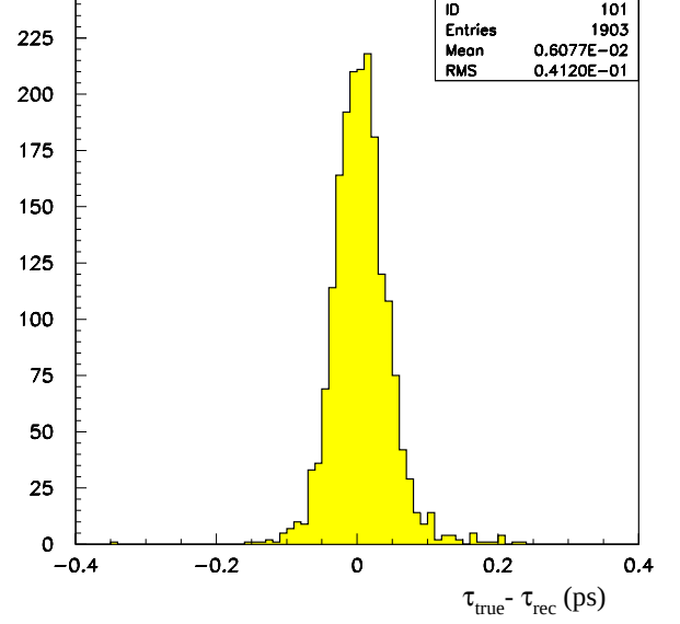
Fig. 9.16: Comparison of the reconstructed and generated B_c lifetime
