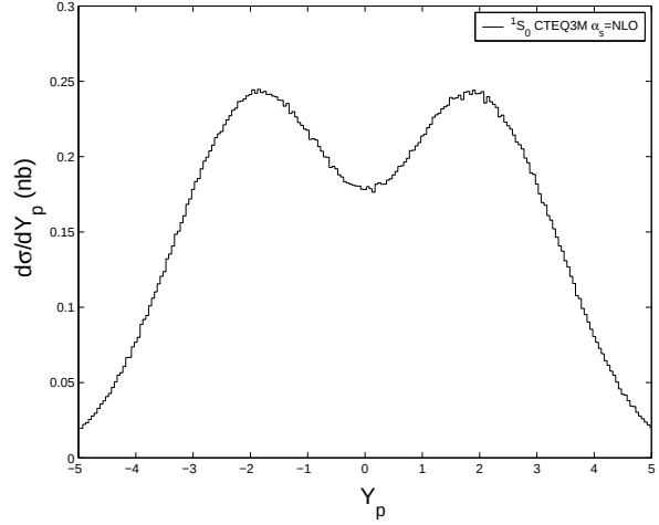
Fig. 9.11: The B_c pseudo-rapidity distribution obtained with the parton distribution function CTEQ3M. For details see Ref. [47].
