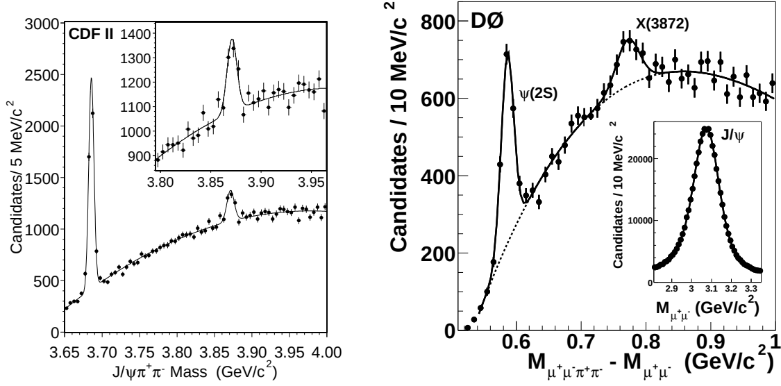
Fig. 3.31: Confirmation of the X(3872) in inclusive p\bar{p} collisions by CDF [463] (left) and D0 [464] (right). In each case peaks due to \psi' and X(3872) \rightarrow \pi^+ \pi^- J/\psi can be clearly seen; the insets show (left) an enlargement of the X(3872) region and (right) the mass distribution for the J/\psi \rightarrow \mu^+ \mu^- candidates used in the analysis.
