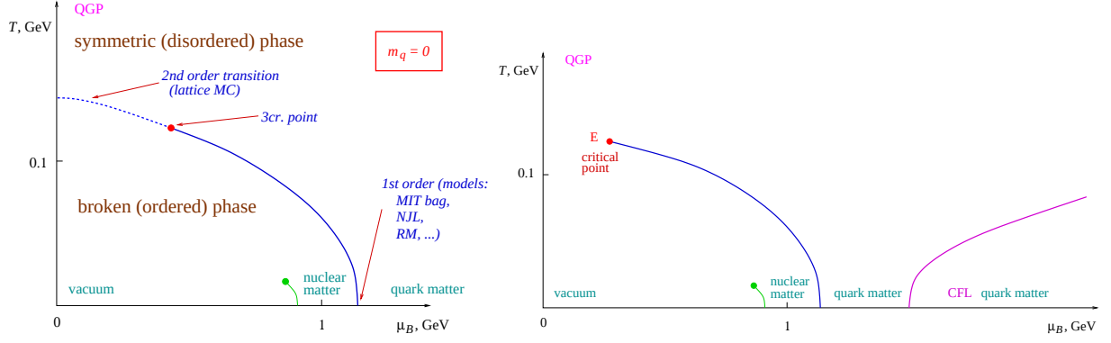
Fig. 7.1: The phase diagram of QCD for two massless flavours (left) and what is expected for realistic values of the quark masses (right). From M. Stephanov [19].
