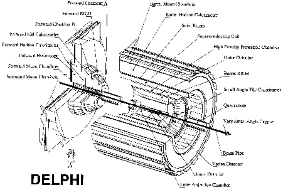
Fig. 2.11: DELPHI detector [15].
