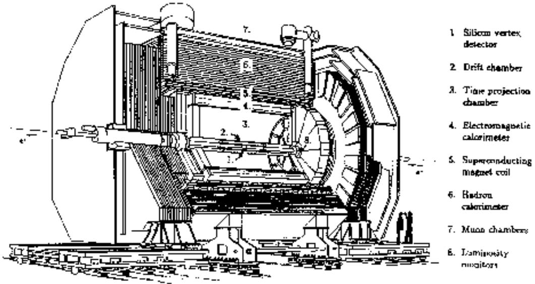
Fig. 2.10: ALEPH detector [14].
