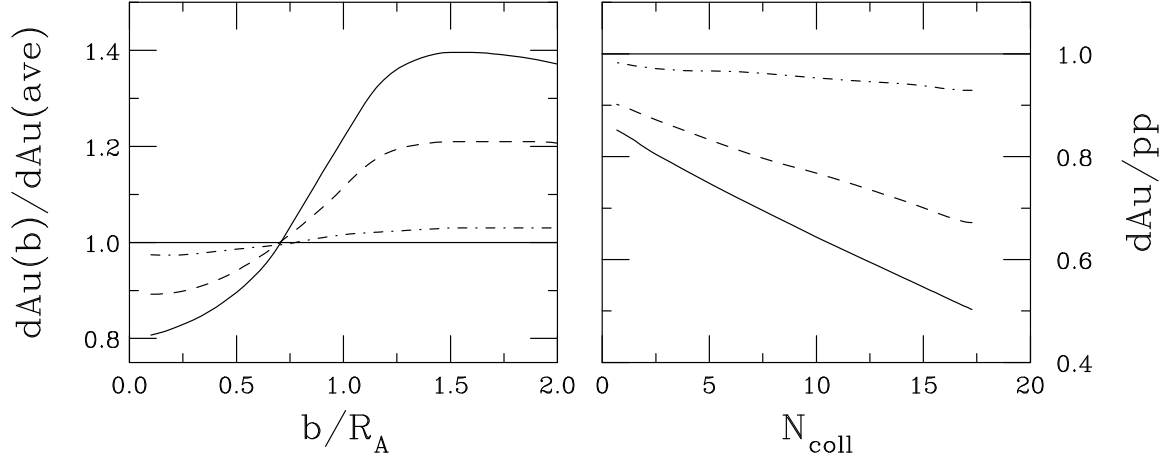
Fig. 7.17: Left-hand side: The J/\psi (dAu(b)/pp)/(dAu(ave)/pp) ratio as a function of b/R_A . Right-hand side: The ratio dAu/pp as a function of N_{coll} . Results are shown for y = -2 (dot-dashed), y = 0 (dashed) and y = 2 (solid) at 200 GeV for a growing octet with \sigma_{abs} = 3 mb and the EKS98 parameterization.
