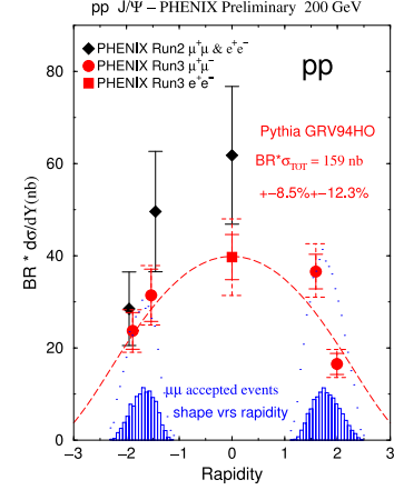
Fig. 7.28: J/\psi differential cross-section, multiplied by the dilepton branching ratio, versus rapidity as measured by the central and muon spectrometers.
