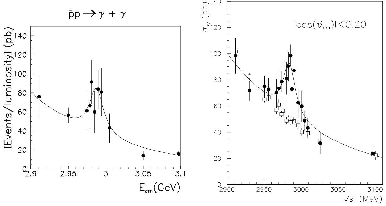
Fig. 3.18: Cross-section (black dots) observed by E760 (left) and E835(right) for the reaction p\bar{p} \rightarrow \gamma\gamma in the region with \cos\theta_{CM} < 0.25 (E760), 0.2 (E835). The blank squares show the expected feed-down from \pi^0\pi^0 , \pi^0\gamma .
