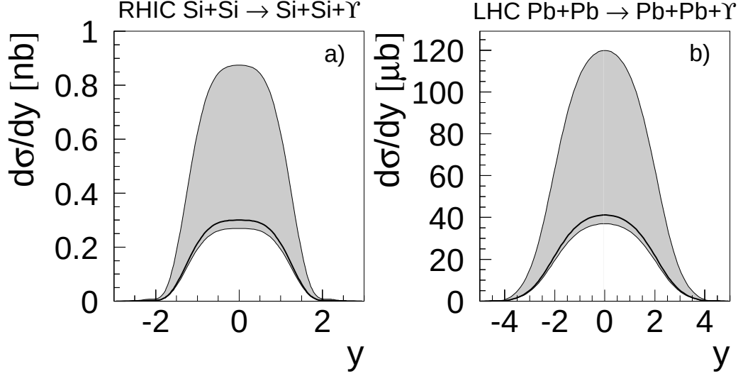
Fig. 7.33: Rapidity distributions of \Upsilon mesons produced in coherent photonuclear interactions at RHIC and the LHC [136]. The solid curves correspond to the parameterization \sigma_{\gamma p}(W_{\gamma p}) = 0.06W_{\gamma p}^{1.7} (pb) and the grey bands show the uncertainty in \sigma_{\gamma p}
