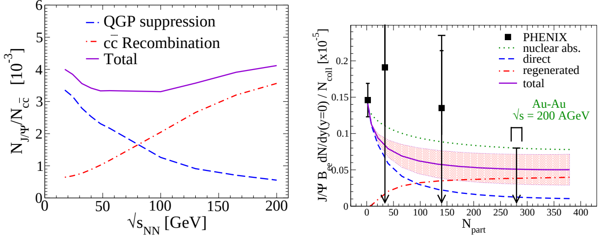
Fig. 7.18: Left-hand side: excitation function of the ratio of J/\psi 's over c\bar{c} pairs in central heavy-ion collisions ( N_{part} = 360 ) from SPS to RHIC energies [104, 105] for the J/\psi yield from quark gluon plasma suppressed primordial production (dashed), secondary J/\psi production from c\bar{c} coalescence (dot-dashed) and the sum (solid). Right-hand side: Centrality dependence of the J/\psi yield, normalized to the number of primordial NN collisions, in Au+Au collisions at RHIC within a kinetic theory framework including in-medium effects on both open and hidden charm states [108]. We show J/\psi suppression with only the loss term in Eq. (7.50) (dashed), secondary J/\psi production (dot-dashed), primordial J/\psi 's subject to nuclear absorption only (dotted) while the band around the solid line, representing the full solution of the rate equation, indicates the uncertainty induced by varying the in-medium masses of open-charm hadrons.
