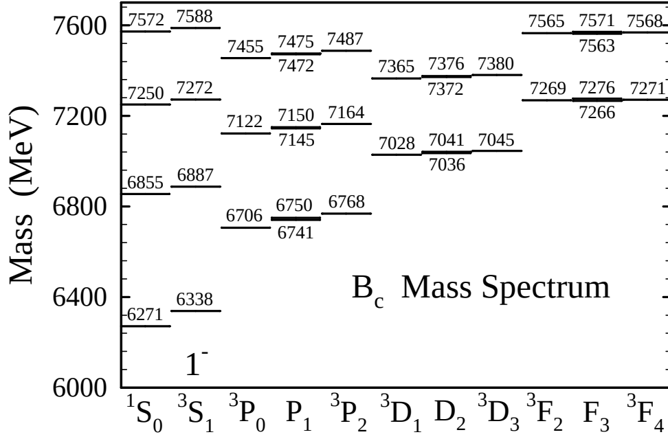
Fig. 3.9: B_c spectrum.
