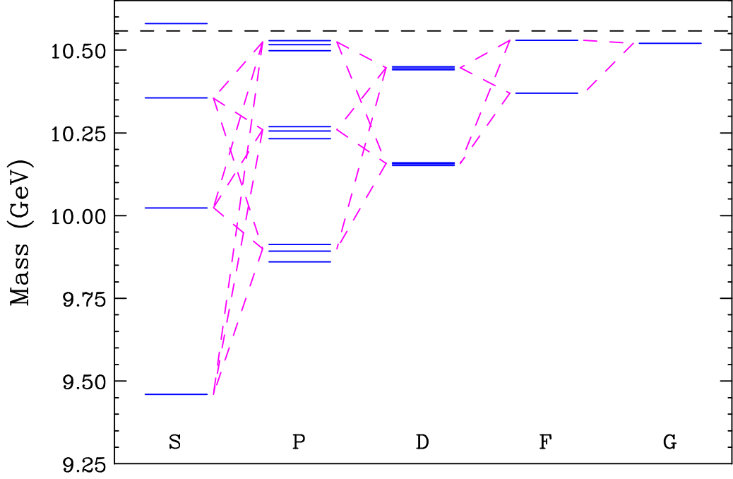
Fig. 4.10: E1 transitions in the narrow spin triplet \bar{b}b states. For each S–P transition indicated there are three individual transitions (one for each P_J state); while for transitions involving any other pair of orbital angular momenta (P–D, D–F, F–G, ...) there are six individual transitions ( \Delta J = 0, \pm 1 ).
