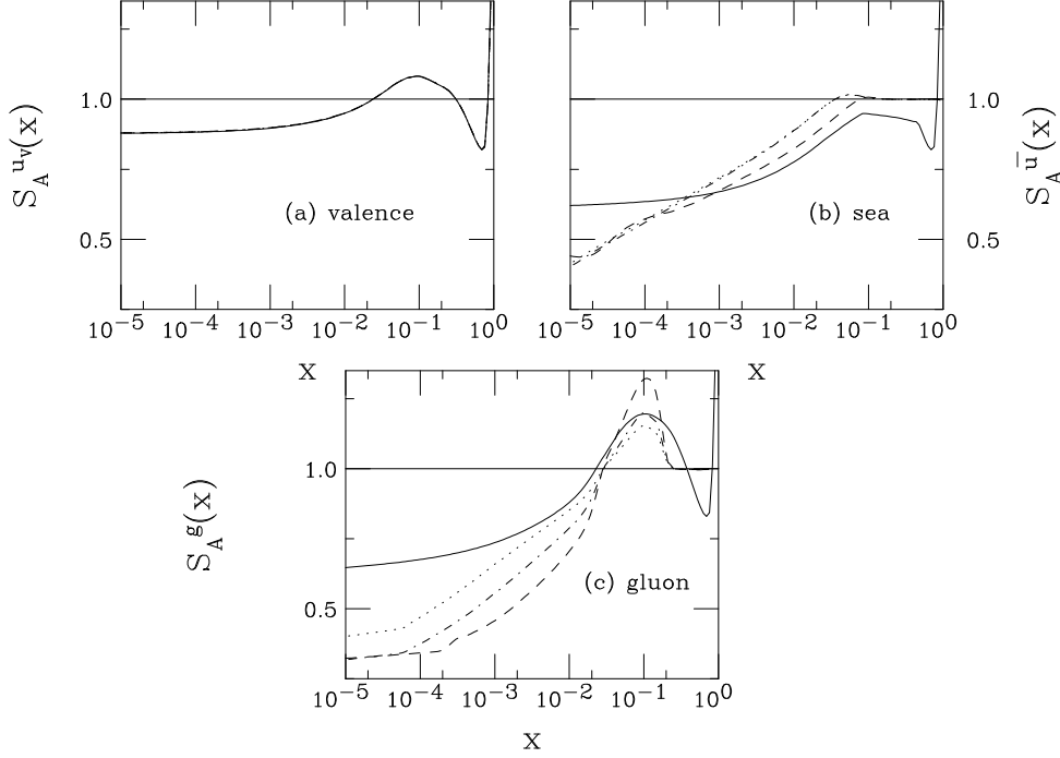
Fig. 7.15: The shadowing parameterizations are compared at the scale \mu = 2m_c = 2.4 GeV. The solid curves are EKS98, the dashed, FGSo, dot-dashed, FGSh, and dotted, FGSI.
