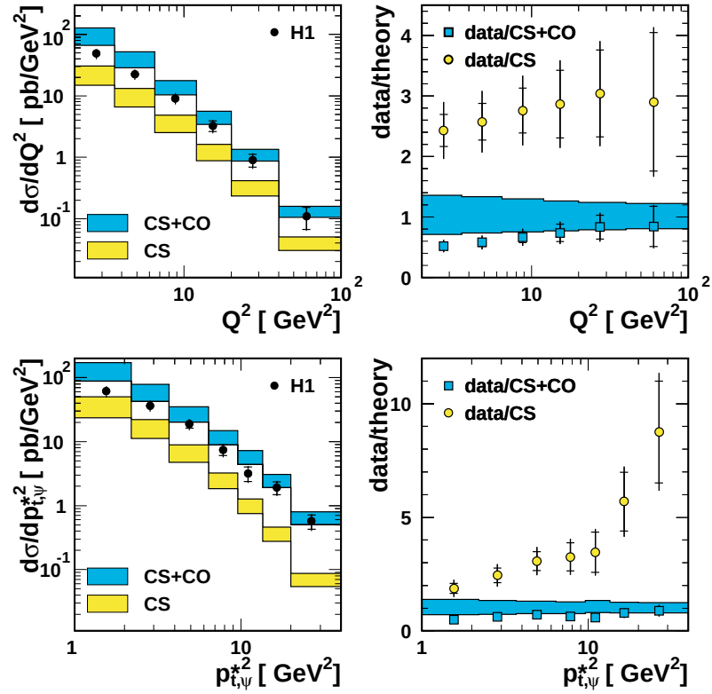
Fig. 5.20: Differential cross-sections d\sigma/dQ^2 (top left panel) and d\sigma/dp_{T,\psi}^{*2} (bottom left panel) and the corresponding ratios of data to theory (right panels). The data from H1 [183] are compared with the NRQCD calculation [182] (CO+CS, dark band) and the colour-singlet contribution [182] (CS, light band).
