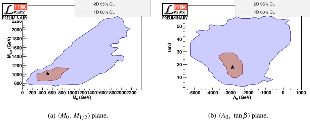
Figure 2: Preferred two-dimensional CMSSM parameter regions. We profile over the remaining fit parameters. The red and blue areas correspond to the one-dimensional 68% C.L. ( \Delta\chi^2 = 1 ) and two-dimensional 95% C.L. ( \Delta\chi^2 = 6.18 ) parameter region, respectively. The black star indicates the best-fit point.
